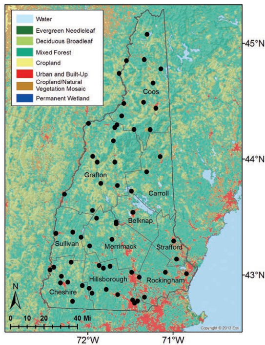
FIGURE 11. Location map for Global Historical Climatology Network (GHCN)-Daily stations (black dots) in New Hampshire with daily precipitation records for the period 1960–2012. Data used to investigate climate change in southern New Hampshire comes from the 41 stations below 43.9°N latitude.
